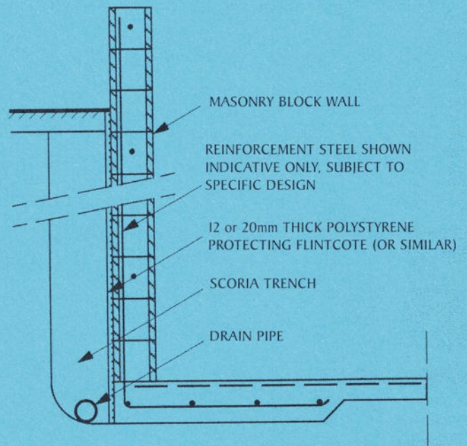
POLYSTYRENE PROTECTION SHEETS - SECTION NOT TO SCALE
