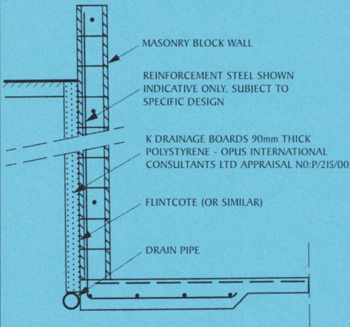
K DRAINAGE BOARD - SECTION NOT TO SCALE
