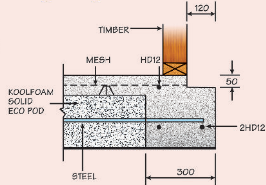
Fig 2 Edge with Brick Veneer
