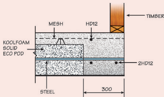
Fig 3 100mm Rib
